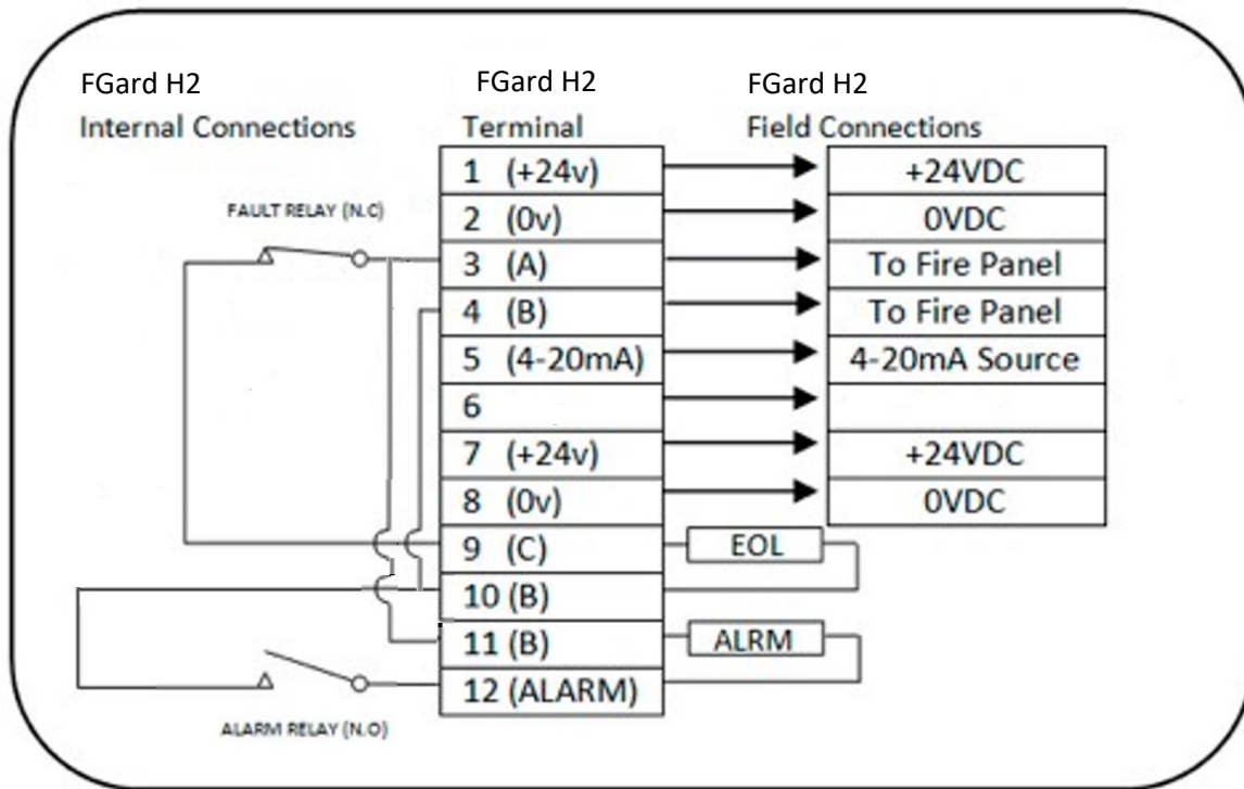
Figure 7: FGard H2 Internal Inter-connections
